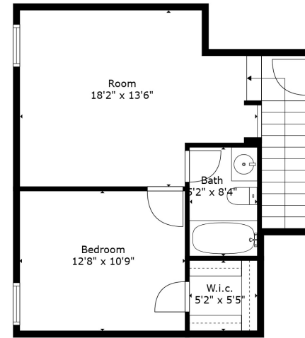
Floor 2
